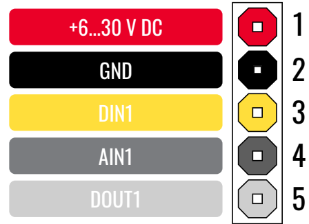
FMB920 pinout
